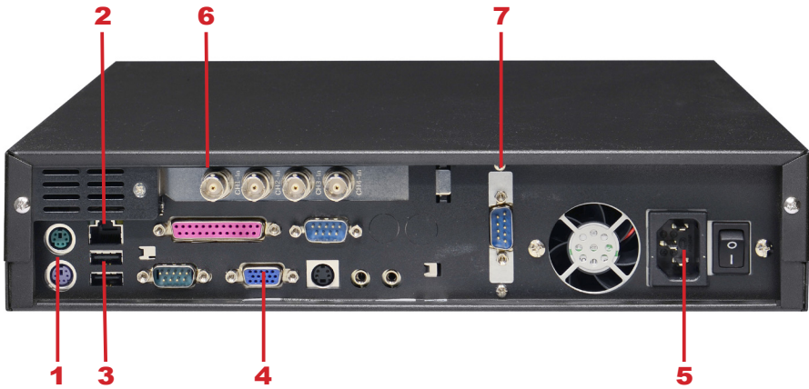
1. PS/2 2. Ethernet 3. USB×2 4. VGA 5. Power Connector 6. Video In x 4 (optional) 7. Audio In (with an extra cable, optional)
